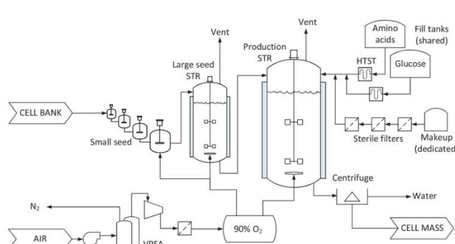
Figure 1. Fed-batch ACBM production system utilized in this LCA of ACBM. This image was taken from Scale-up economics for cultured meat (Humbrid, 2021)
