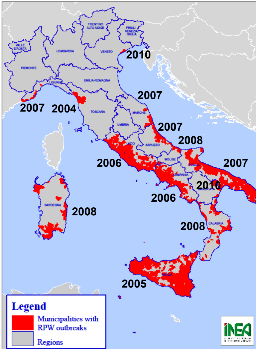
Map of Municipalities where RPW has been detected Update: February 2013
